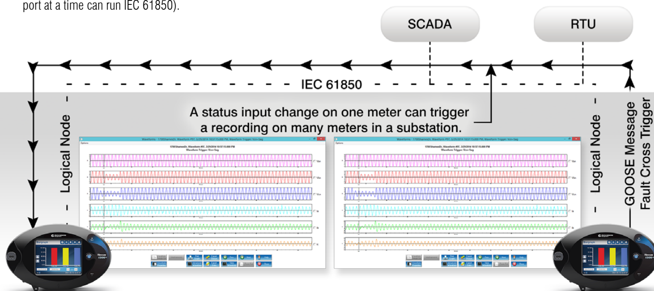
Fault-based cross trigger waveforms based on GOOSE messages
